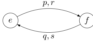
Figure 8.3: The condition (K).
