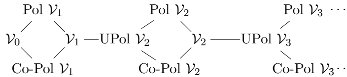
Figure 10.5: The Straubing-Thérien hierarchy
