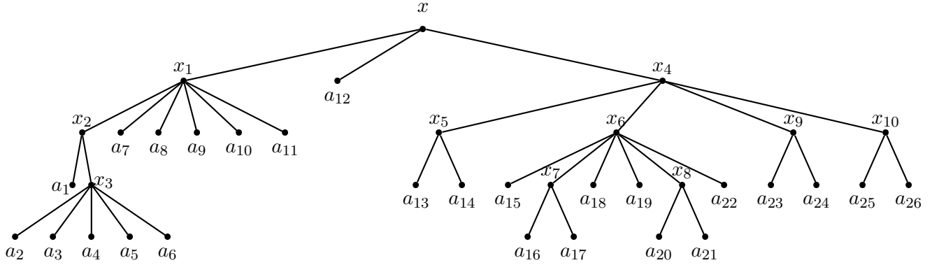
Figure 4.1: The tree t(x) .
