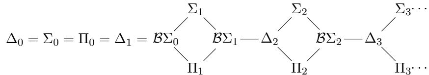
Figure 10.4: The logical hierarchy
